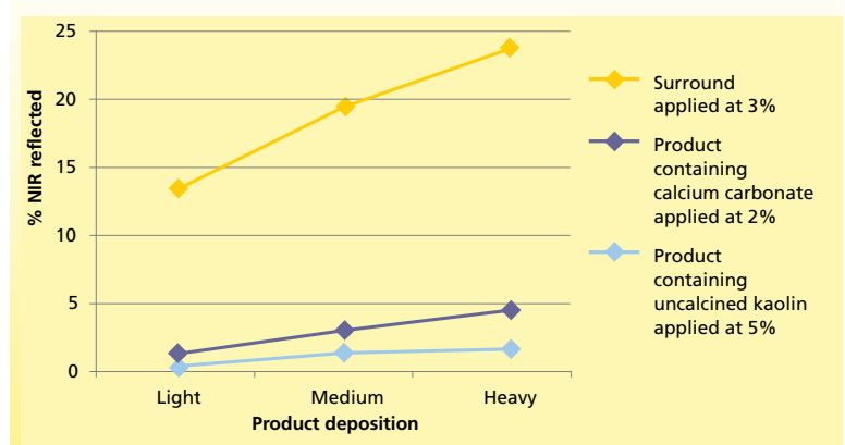
Graph 3. Relative reflectance of NIR at a range of deposition levels.
